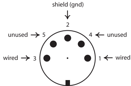
Figure 1—MIDI cable with connectors showing pin-out
